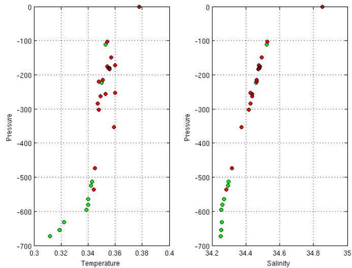
Warning Objective Analysis Anomalies 2017 March TEMP PSAL - DAC KO
