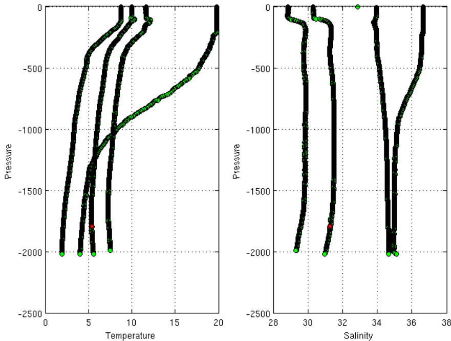
Warning Objective Analysis Anomalies 2017 March TEMP PSAL - DAC ME
