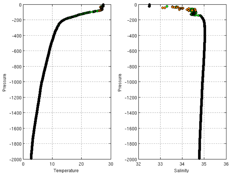
Warning Objective Analysis Anomalies 2017 March TEMP PSAL - DAC IN
