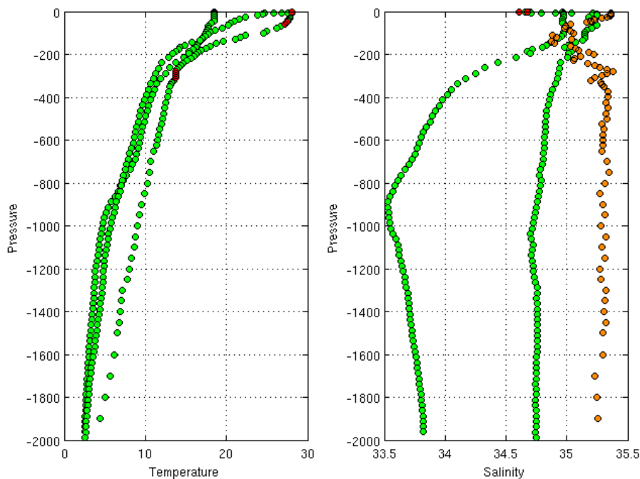
Warning Objective Analysis Anomalies 2017 March TEMP PSAL - DAC HZ
