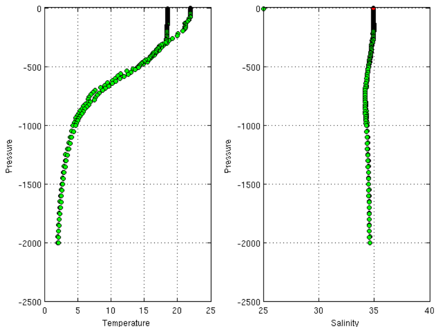
Warning Objective Analysis Anomalies 2017 March TEMP PSAL - DAC JA
