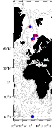
Warning Objective Analysis Anomalies 2017 March
