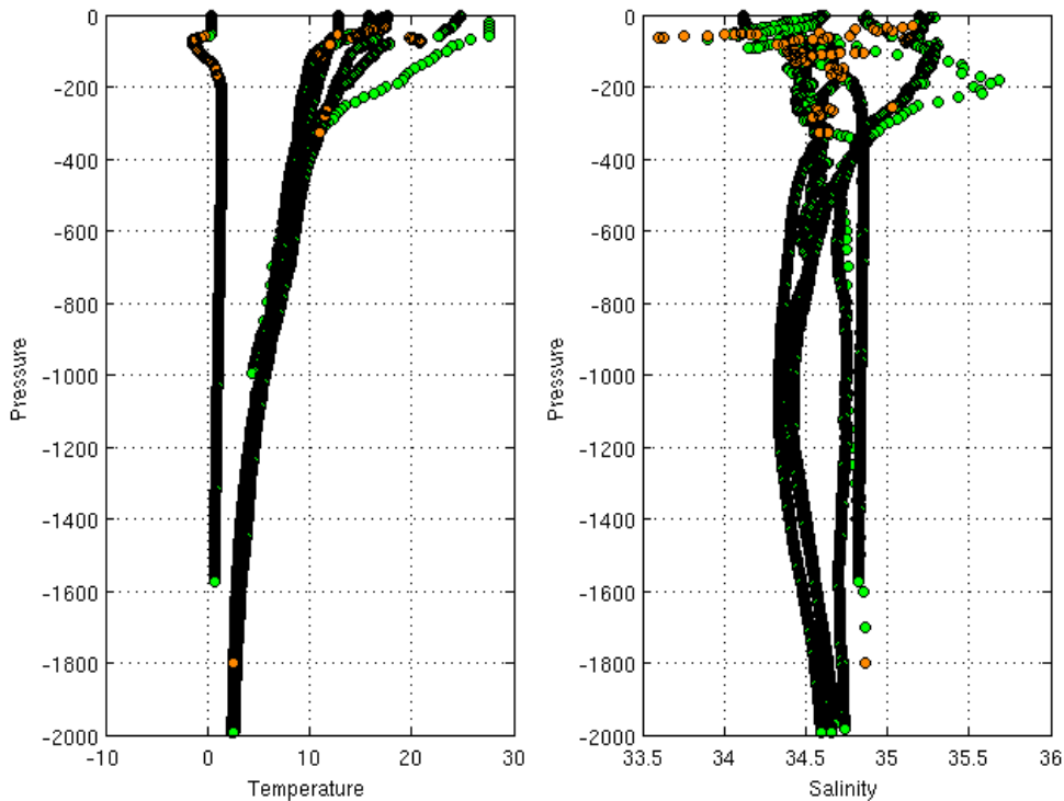
Warning Objective Analysis Anomalies 2017 March TEMP PSAL - DAC CS
