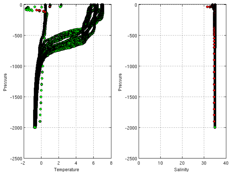
Warning Objective Analysis Anomalies 2017 March TEMP PSAL - DAC BO
