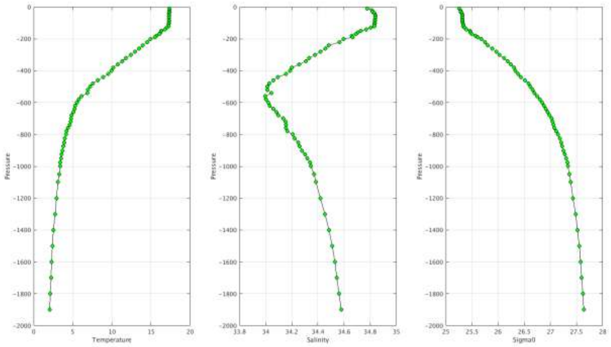
Warning Objective Analysis Anomalies 2018 April TEMP PSAL : DAC KO- Float 2901779 - 29
