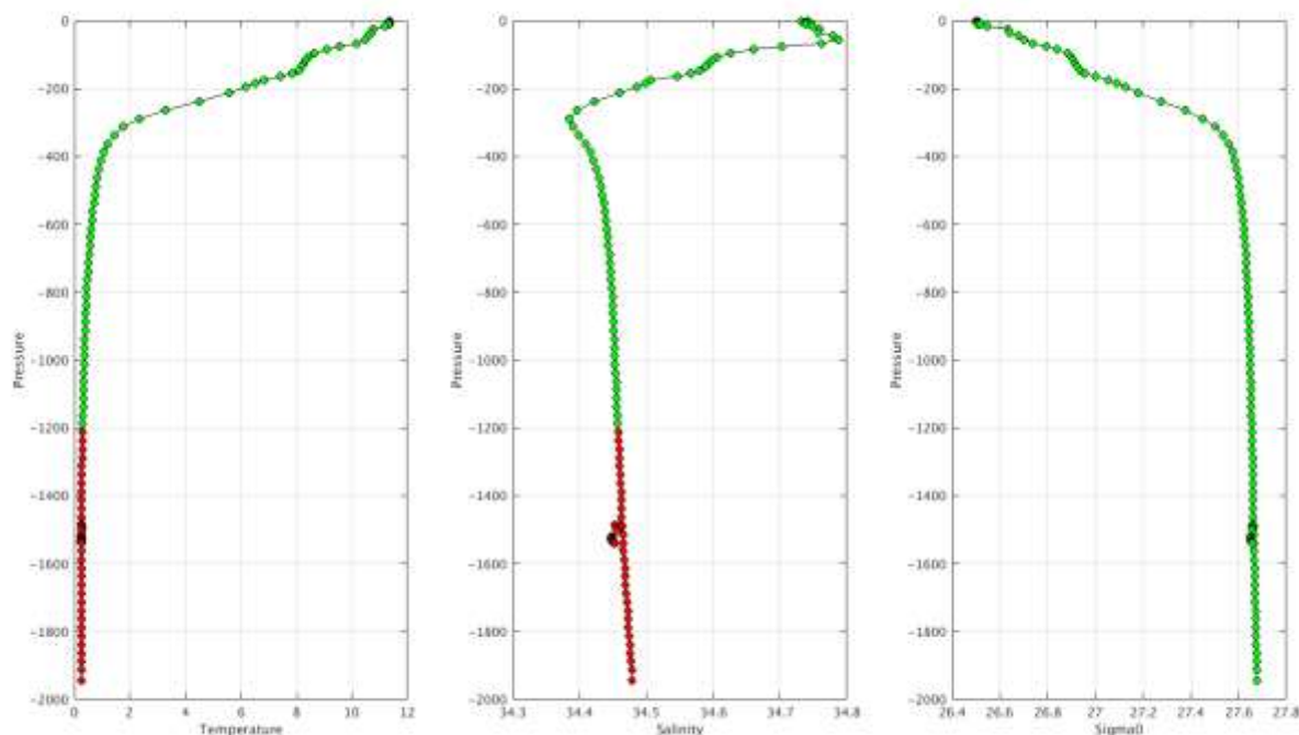
Warning Objective Analysis Anomalies 2018 April TEMP PSAL : DAC KM- Float 2901759 - 61
