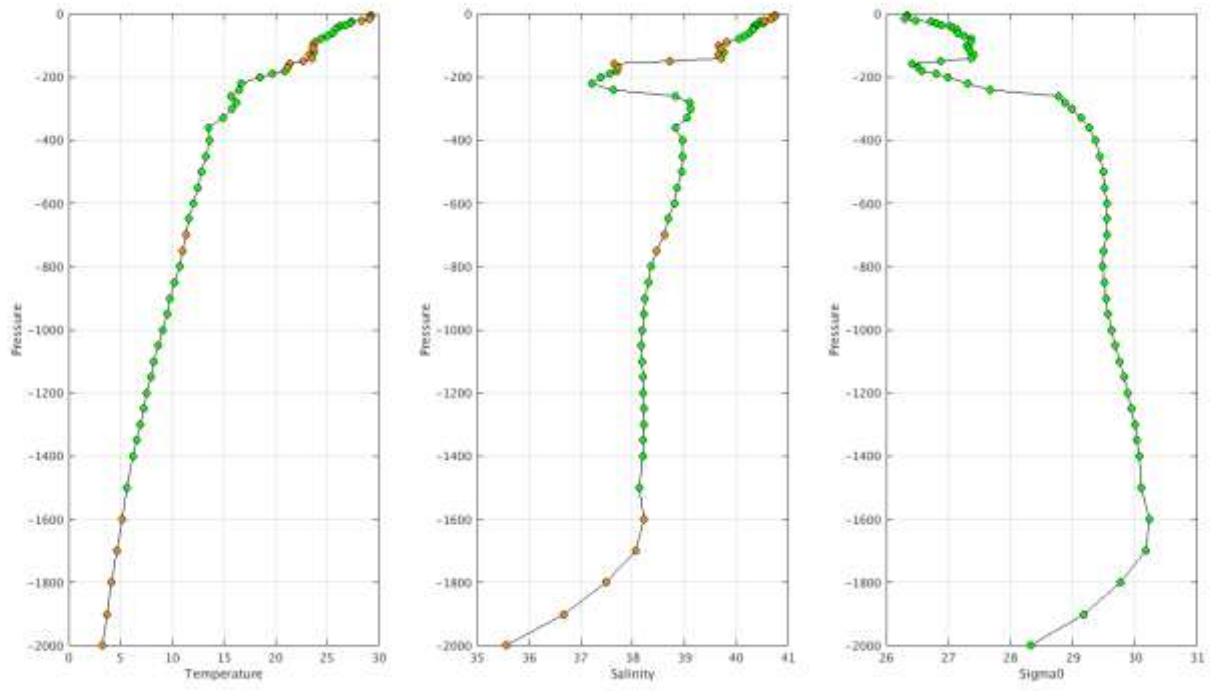
Warning Objective Analysis Anomalies 2018 April TEMP PSAL : DAC IN- Float 2902206 - 78
