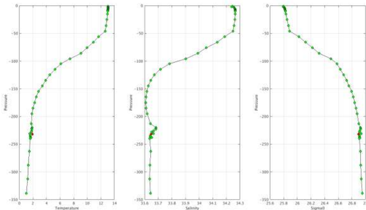
Warning Objective Analysis Anomalies 2018 April TEMP PSAL : DAC KM- Float 2901724 - 192
