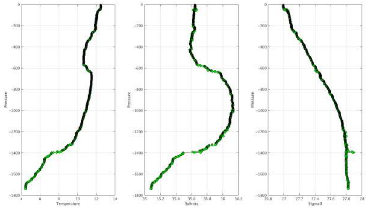
Warning Objective Analysis Anomalies 2018 April TEMP PSAL : DAC BO- Float 3901909 - 48
