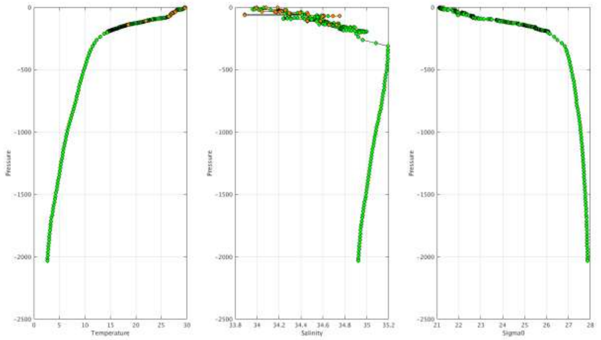
Warning Objective Analysis Anomalies 2018 April TEMP PSAL : DAC IN- Float 2902233 - 153
