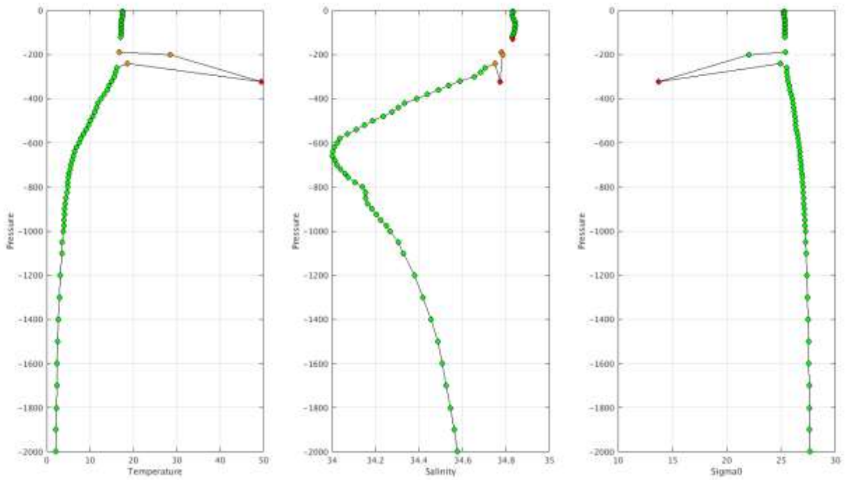
Warning Objective Analysis Anomalies 2018 April TEMP PSAL : DAC KO- Float 2901779 - 32
