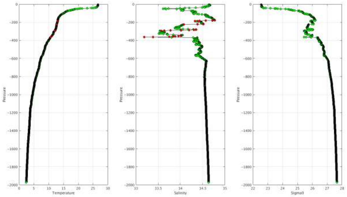
Warning Objective Analysis Anomalies 2018 May TEMP PSAL : DAC AO- Float 3901203 - 79
