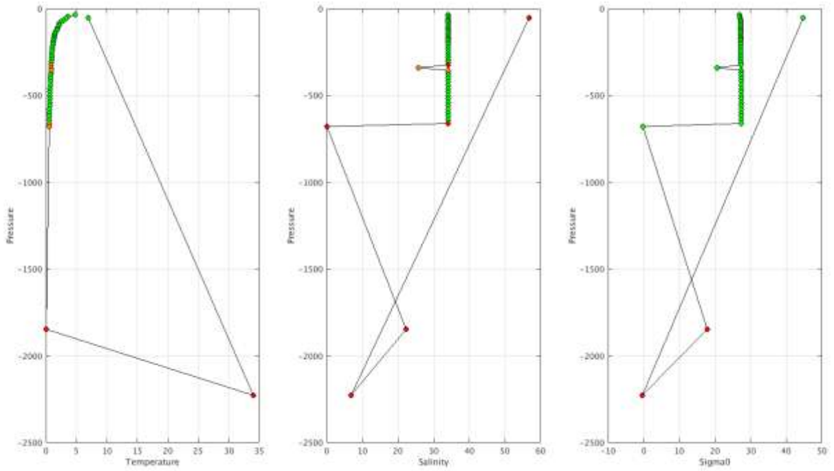
Warning Objective Analysis Anomalies 2018 May TEMP PSAL : DAC RD- Float 2900451 - 498
