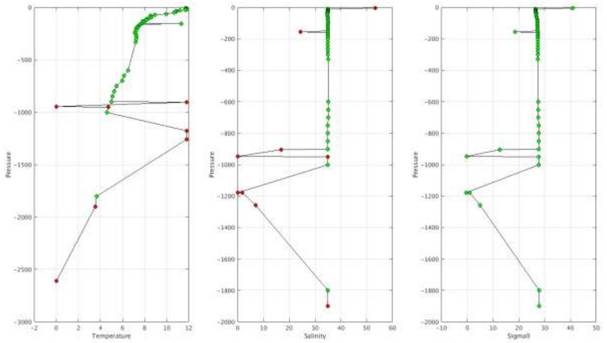
Warning Objective Analysis Anomalies 2018 May TEMP PSAL : DAC BO- Float 6901170 - 114
