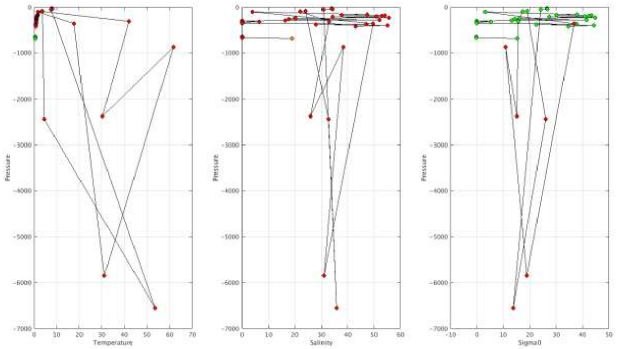
Warning Objective Analysis Anomalies 2018 May TEMP PSAL : DAC RD- Float 2901206 - 302
