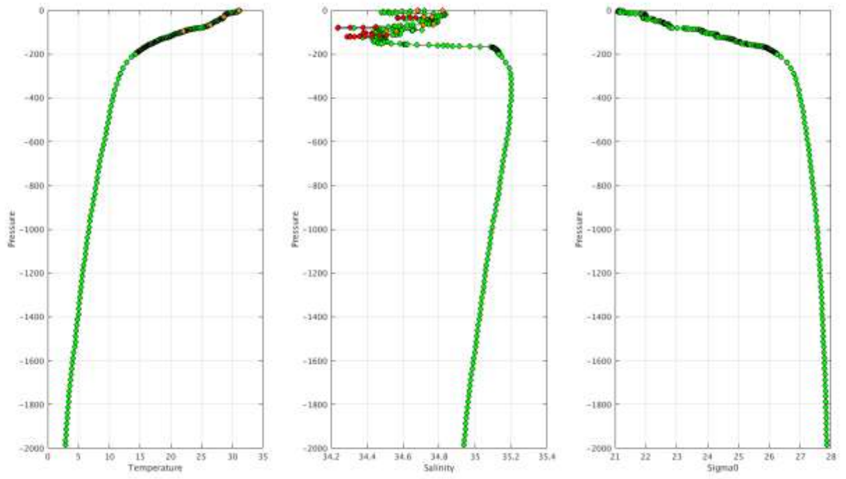
Warning Objective Analysis Anomalies 2018 May TEMP PSAL : DAC IN- Float 2902233 - 159
