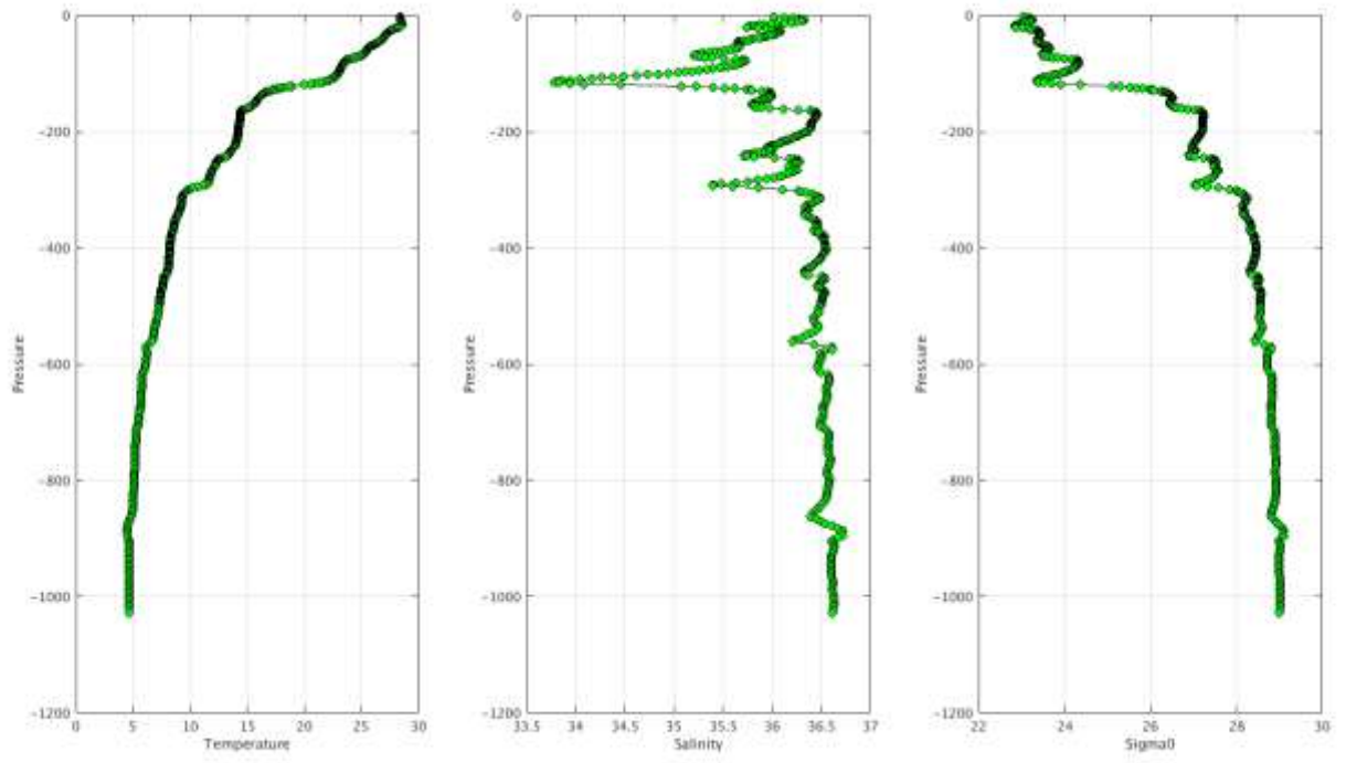
Warning Objective Analysis Anomalies 2018 May TEMP PSAL : DAC BO- Float 3901981 - 2
