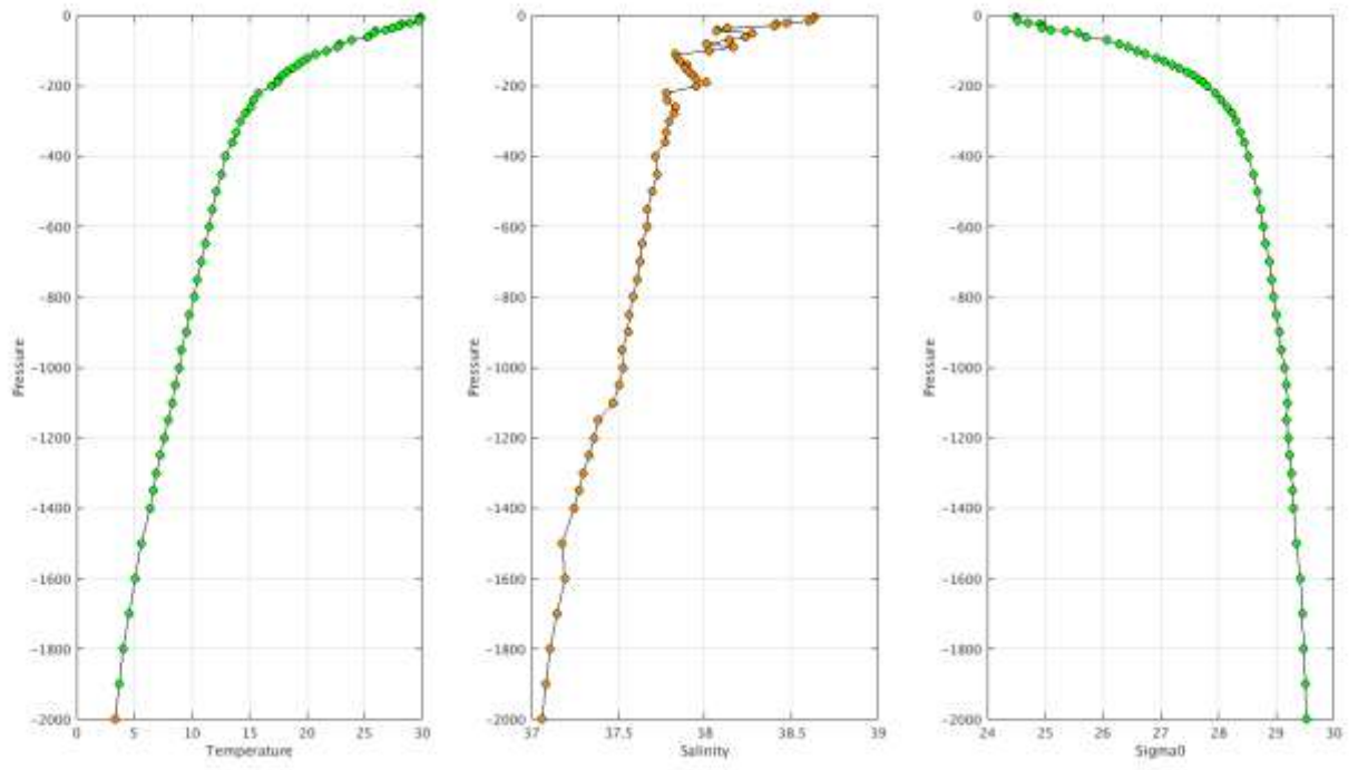
Warning Objective Analysis Anomalies 2018 May TEMP PSAL : DAC IN- Float 2902203 - 79
