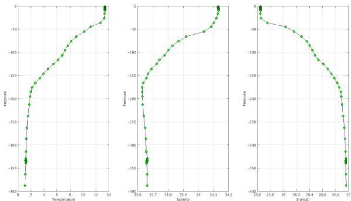
Warning Objective Analysis Anomalies 2018 May TEMP PSAL : DAC KM- Float 2901724 - 196
