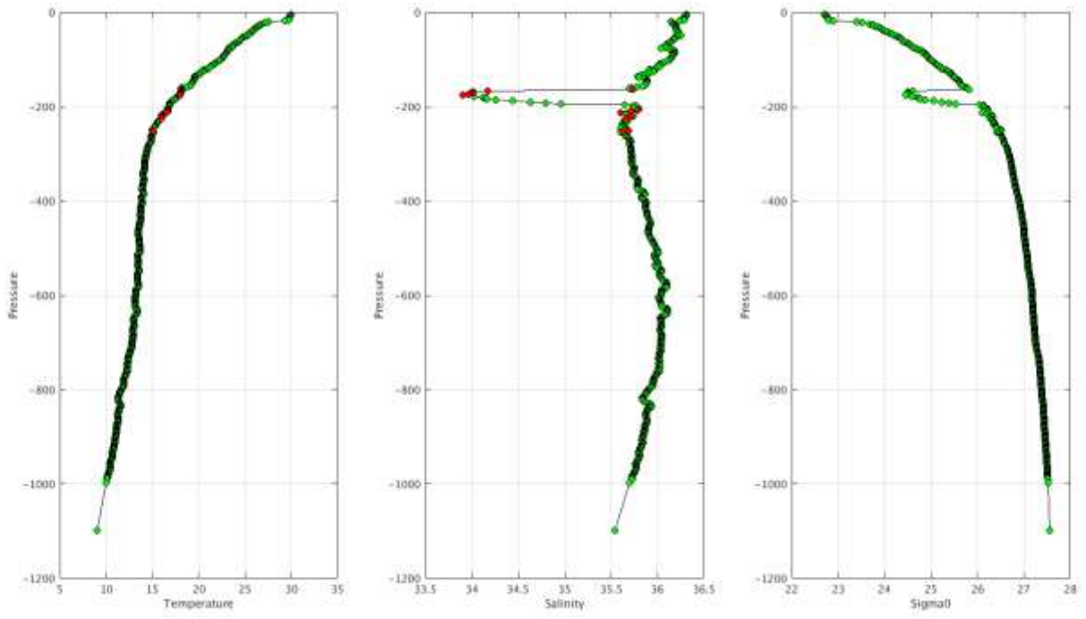
Warning Objective Analysis Anomalies 2018 May TEMP PSAL : DAC AO- Float 2902403 - 156
