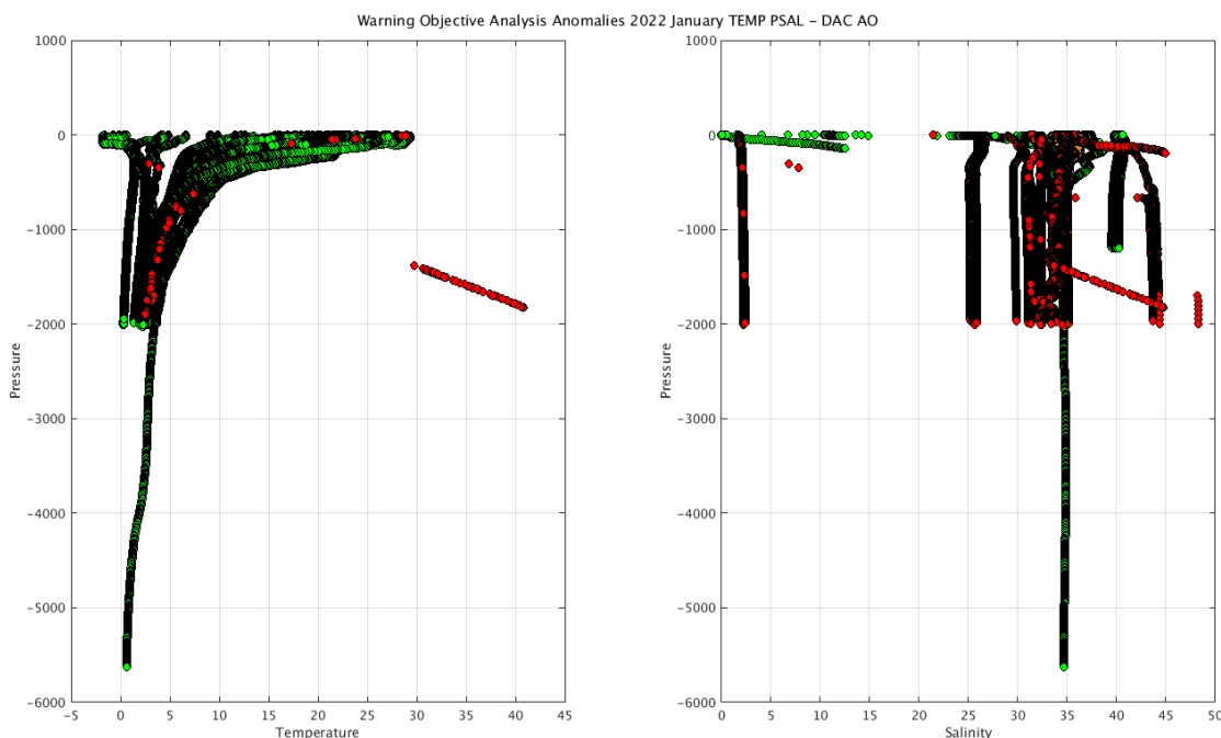
Plot for the 150 first profiles.
