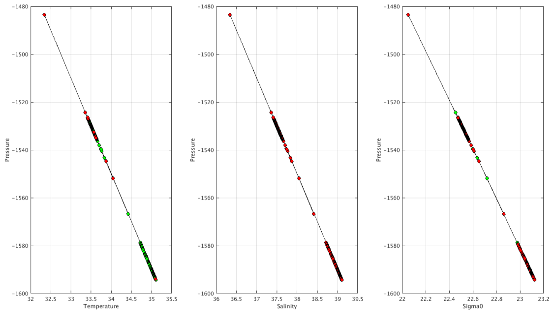
Warning Objective Analysis Anomalies 2022 January TEMP PSAL : DAC AO- Float 4902911 - 154
