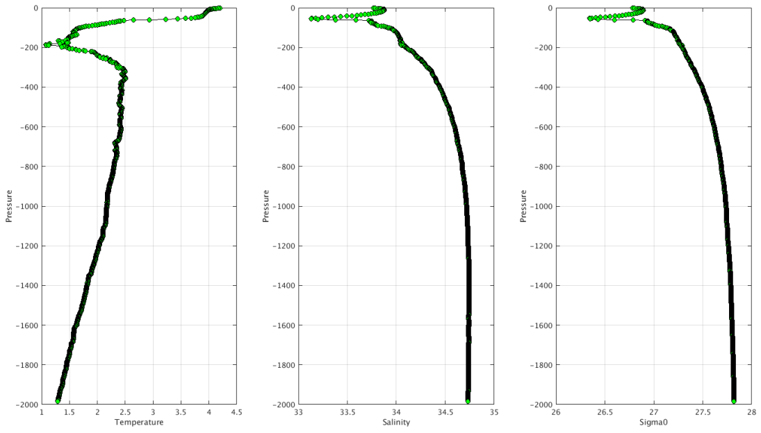
Warning Objective Analysis Anomalies 2022 January TEMP PSAL : DAC AO- Float 1901831 - 227
