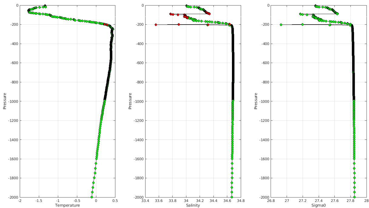
Warning MinMax Anomalies 2023 December TEMP PSAL : DAC BO- Float 1902089 - 35
