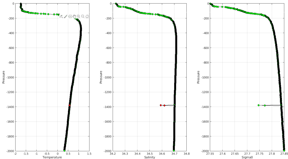
Warning MinMax Anomalies 2023 December TEMP PSAL : DAC CS- Float 7900625 - 213
