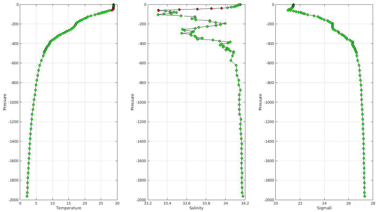
Warning MinMax Anomalies 2023 December TEMP PSAL : DAC KO- Float 3902470 - 44
