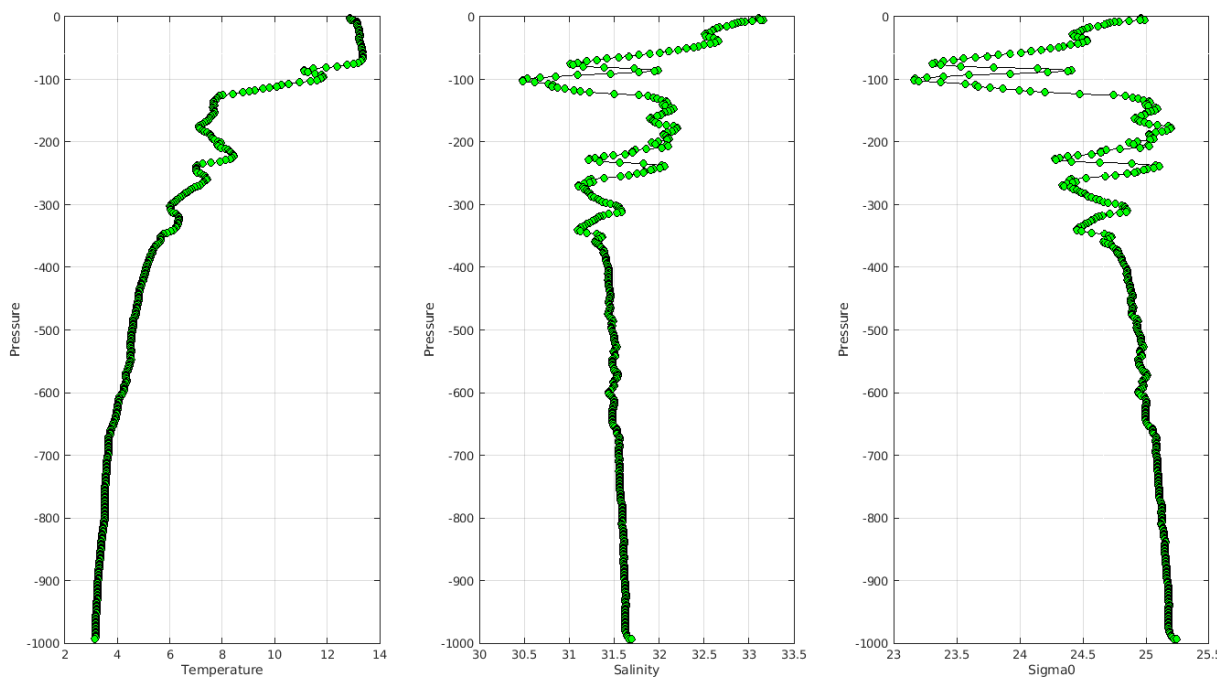
Warning MinMax Anomalies 2023 December TEMP PSAL : DAC BO- Float 6904186 - 34
