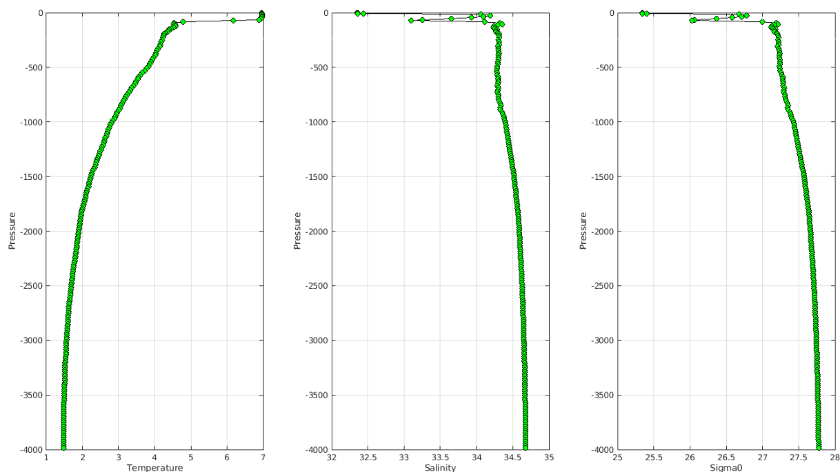
Warning MinMax Anomalies 2023 December TEMP PSAL : DAC ME- Float 4902637 - 15
