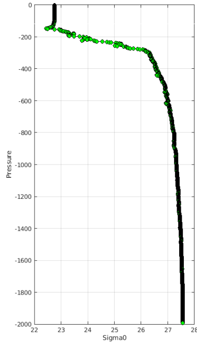
Warning MinMax Anomalies 2023 December TEMP PSAL : DAC JA- Float 5905853 - 177
