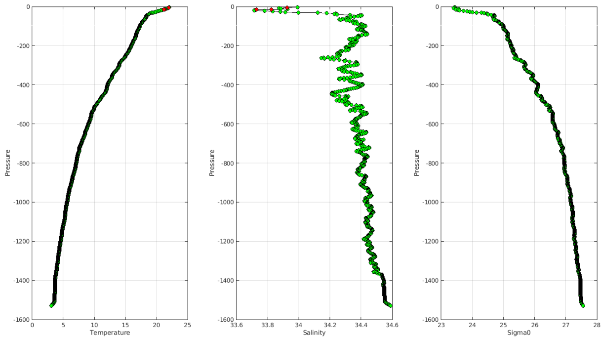
Warning MinMax Anomalies 2023 December TEMP PSAL : DAC CS- Float 5905438 - 156
