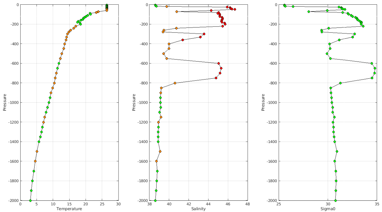
Warning MinMax Anomalies 2023 December TEMP PSAL : DAC IN- Float 2902201 - 285
