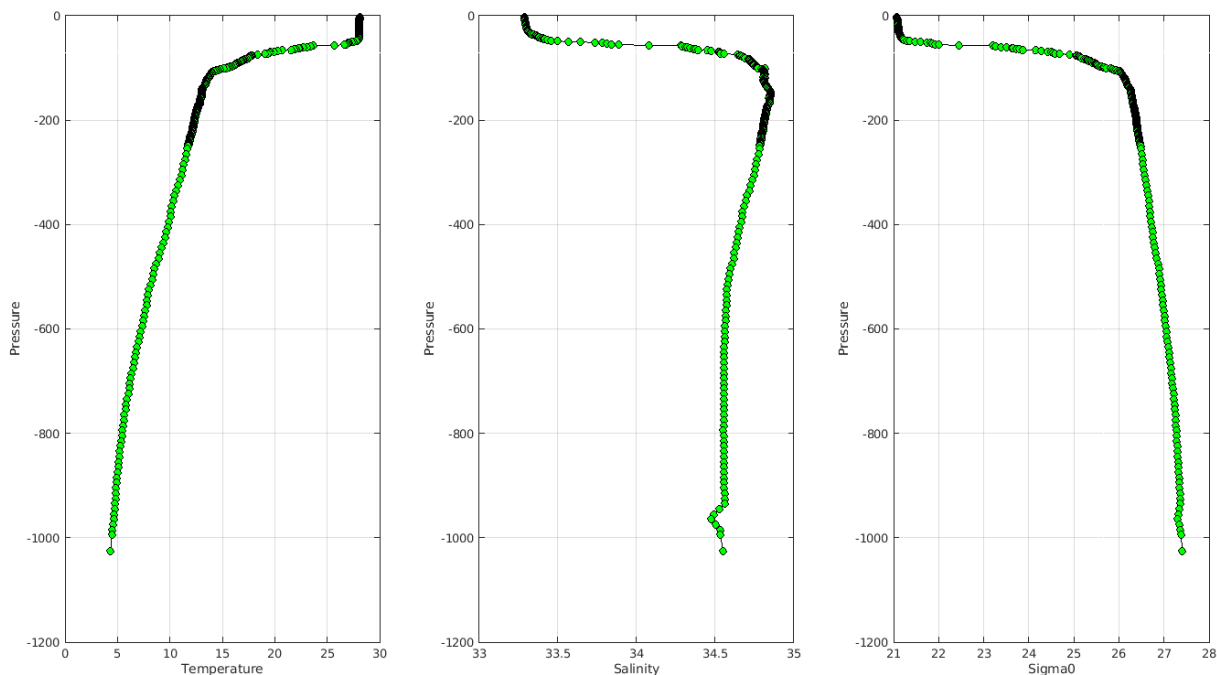
Warning MinMax Anomalies 2023 June TEMP PSAL : DAC BO- Float 3901530 - 124
