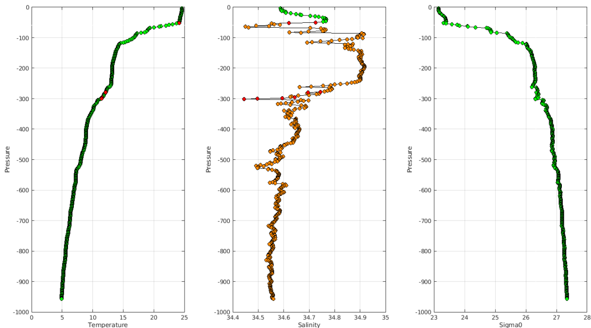
Warning MinMax Anomalies 2023 June TEMP PSAL : DAC AO- Float 3901179 - 163
