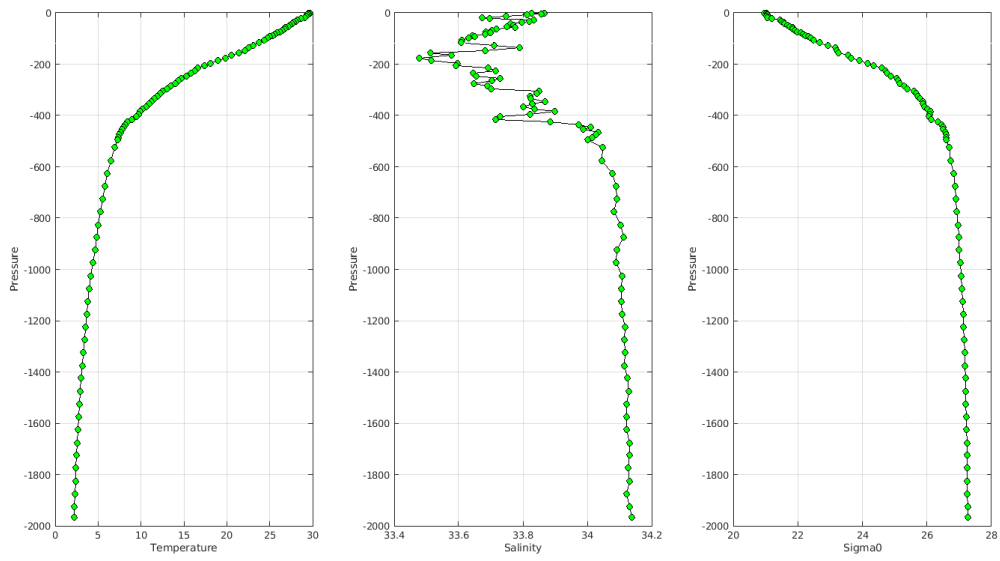
Warning MinMax Anomalies 2023 June TEMP PSAL : DAC KO- Float 3902470 - 26
