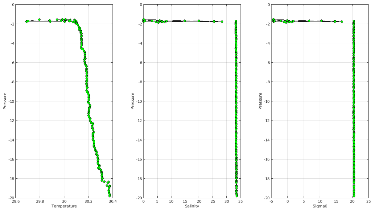
Warning MinMax Anomalies 2023 June TEMP PSAL : DAC AO- Float 3902297 - 14
