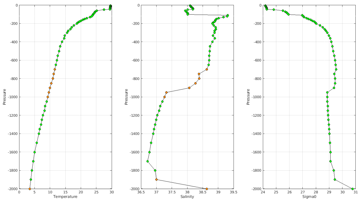
Warning MinMax Anomalies 2023 June TEMP PSAL : DAC IN- Float 2902201 - 267
