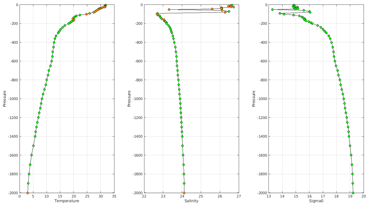
Warning MinMax Anomalies 2023 June TEMP PSAL : DAC IN- Float 2902203 - 265
