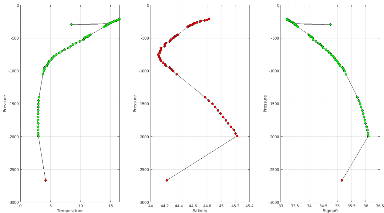
Warning MinMax Anomalies 2023 June TEMP PSAL : DAC BO- Float 3902400 - 90
