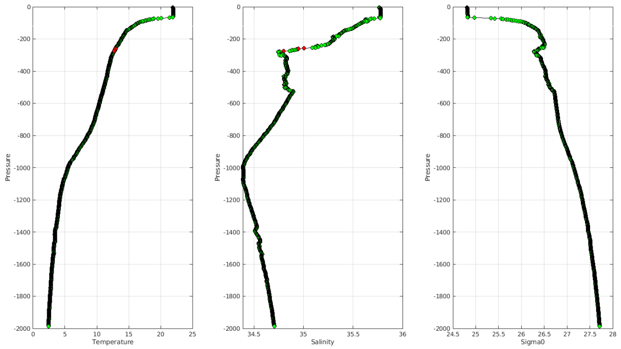
Warning MinMax Anomalies 2023 June TEMP PSAL : DAC CS- Float 1901740 - 161
