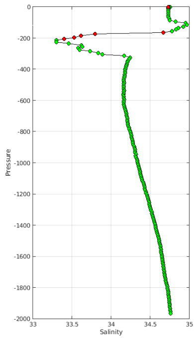
Warning MinMax Anomalies 2023 June TEMP PSAL : DAC HZ- Float 2902835 - 55
