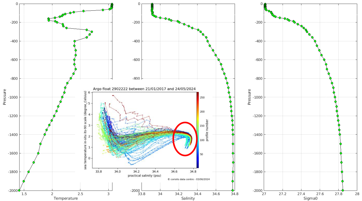
Warning MinMax Anomalies 2024 May TEMP PSAL : DAC IN- Float 2902222 - 269
