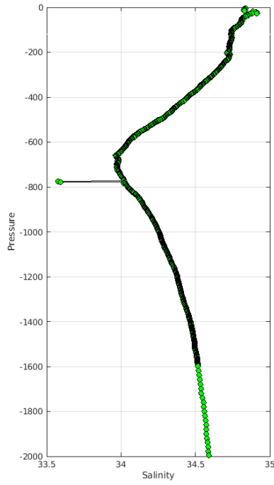
Warning MinMax Anomalies 2024 May TEMP PSAL : DAC JA- Float 2903656 - 5
