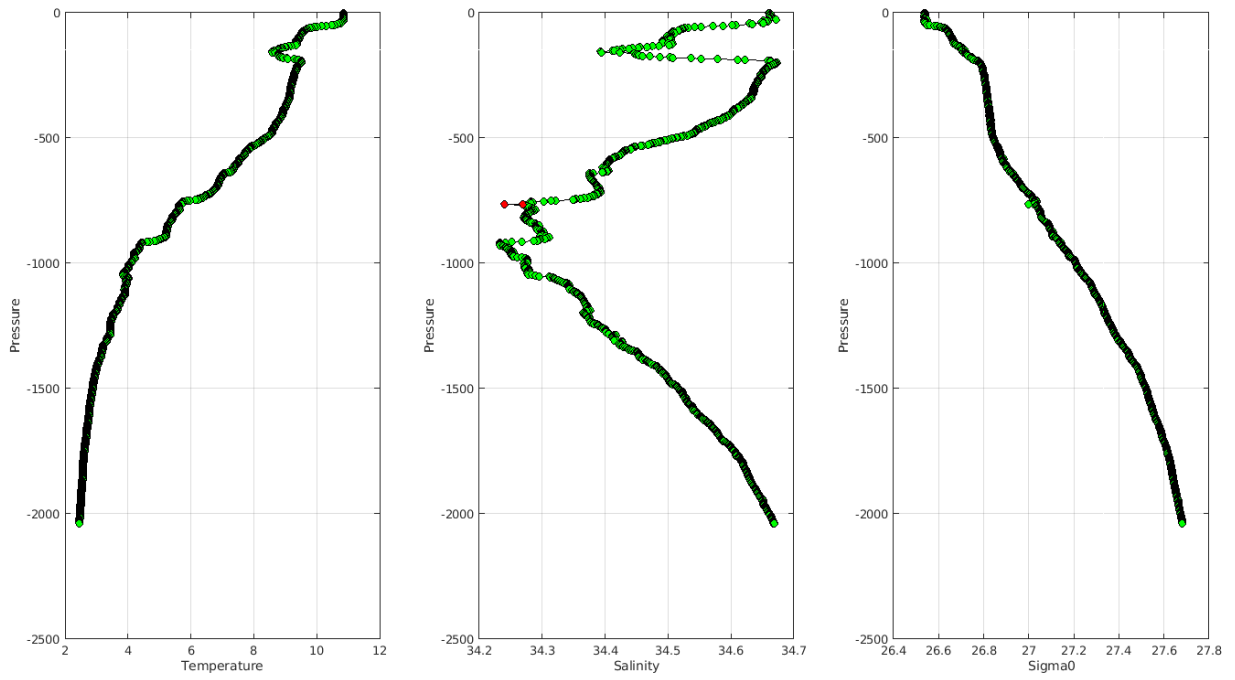
Warning MinMax Anomalies 2024 May TEMP PSAL : DAC CS- Float 5905558 - 8
