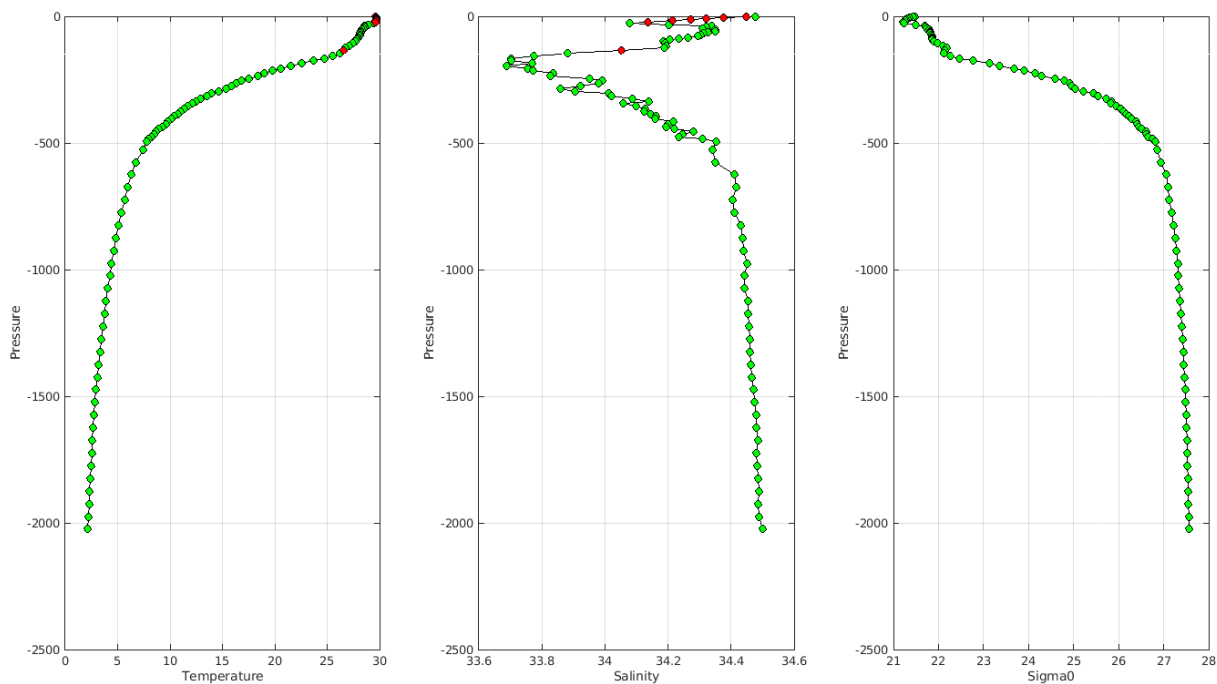
Warning MinMax Anomalies 2024 May TEMP PSAL : DAC KO- Float 3902470 - 60
