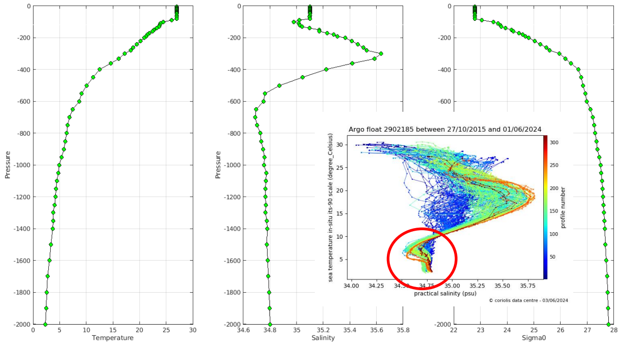
Warning MinMax Anomalies 2024 May TEMP PSAL : DAC IN- Float 2902185 - 314
