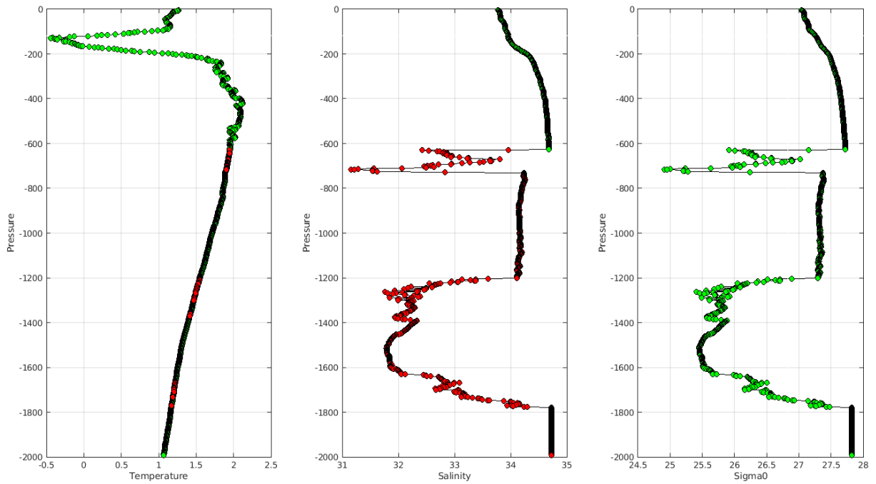
Warning MinMax Anomalies 2024 May TEMP PSAL : DAC CS- Float 7900648 - 151
