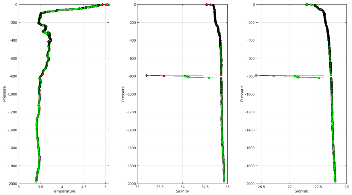
Warning MinMax Anomalies 2024 May TEMP PSAL : DAC ME- Float 4902591 - 73
