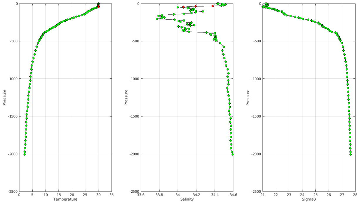
Warning MinMax Anomalies 2024 July_August_withoutCORA TEMP PSAL : DAC KO- Float 3902470 - 72
