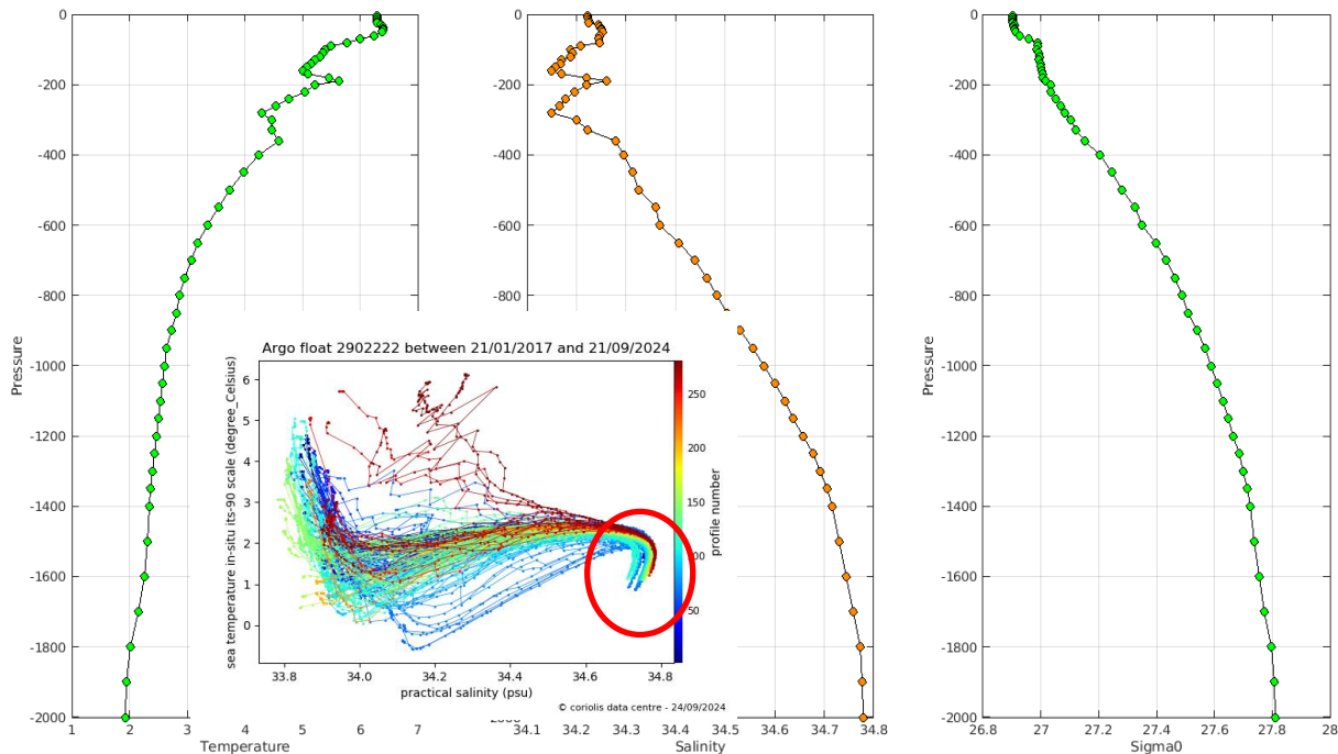
Warning MinMax Anomalies 2024 July_August_withoutCORA TEMP PSAL : DAC IN- Float 2902222 - 279
