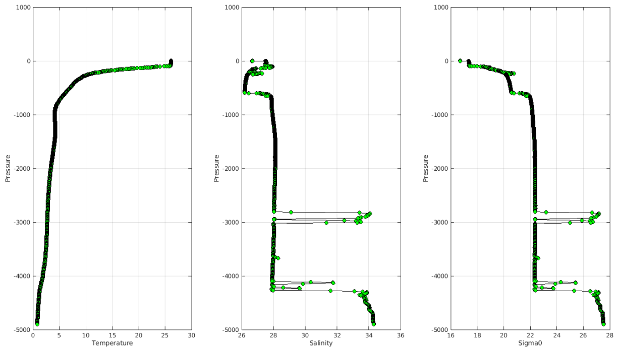
Warning MinMax Anomalies 2024 July_August_withoutCORA TEMP PSAL : DAC AO- Float 3902150 - 206
