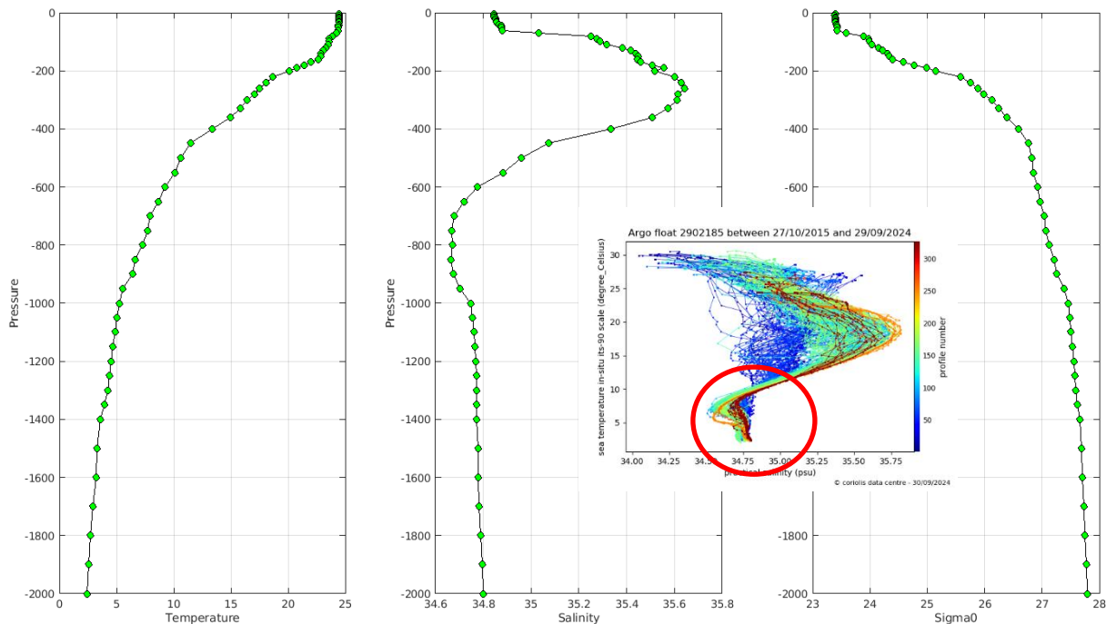
Warning MinMax Anomalies 2024 July_August_withoutCORA TEMP PSAL : DAC IN- Float 2902185 - 326
