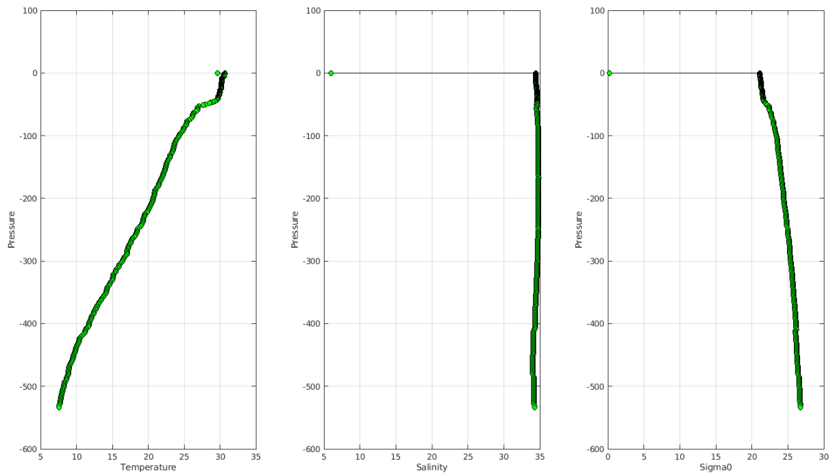
Warning MinMax Anomalies 2024 July_August_withoutCORA TEMP PSAL : DAC JA- Float 5906392 - 327
