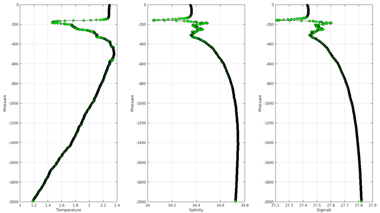
Warning MinMax Anomalies 2024 July_August_withoutCORA TEMP PSAL : DAC CS- Float 7900921 - 130
