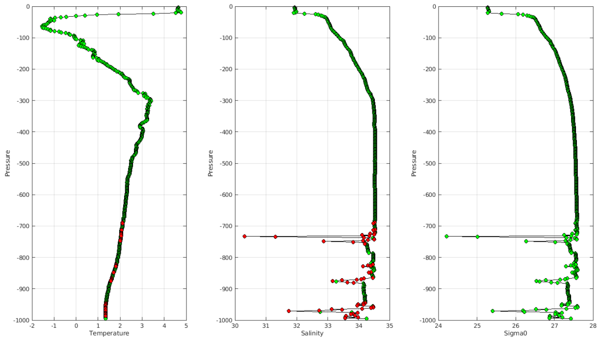
Warning MinMax Anomalies 2024 July_August_withoutCORA TEMP PSAL : DAC AO- Float 1902655 - 86
