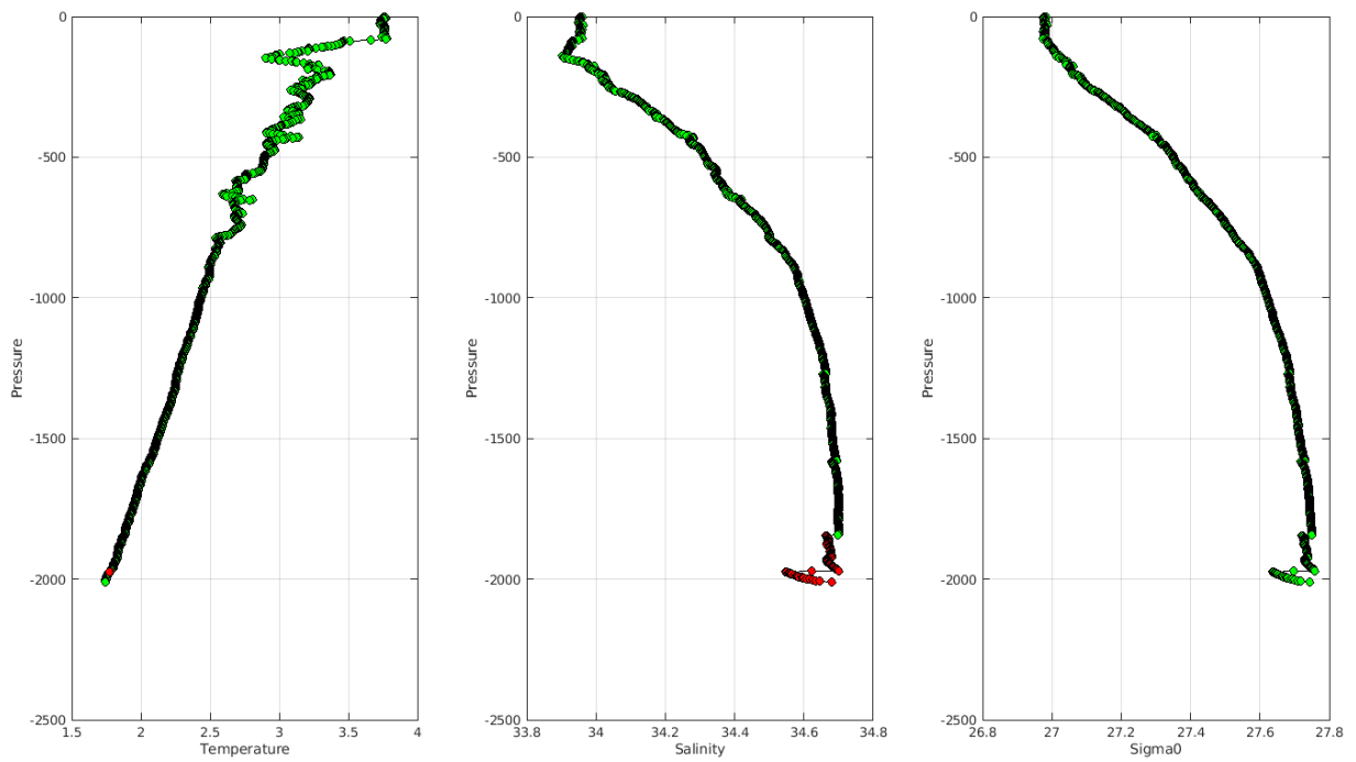
Warning MinMax Anomalies 2024 July_August_withoutCORA TEMP PSAL : DAC CS- Float 5905559 - 23
