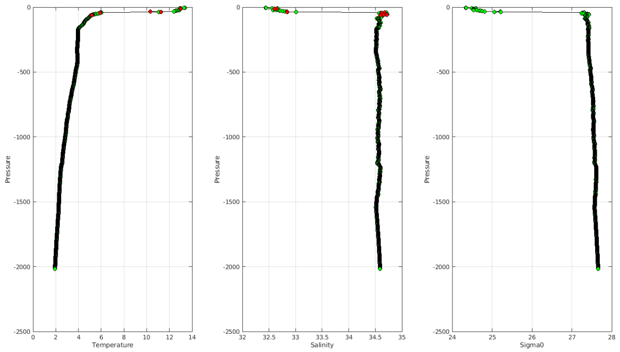
Warning MinMax Anomalies 2024 July_August_withoutCORA TEMP PSAL : DAC JA- Float 2903662 - 124
