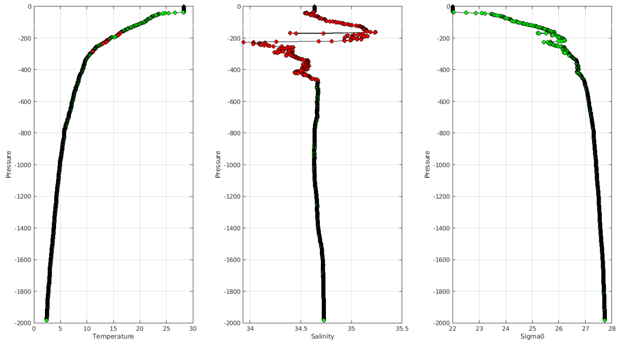
Warning MinMax Anomalies 2024 April TEMP PSAL : DAC CS- Float 5905532 - 52
