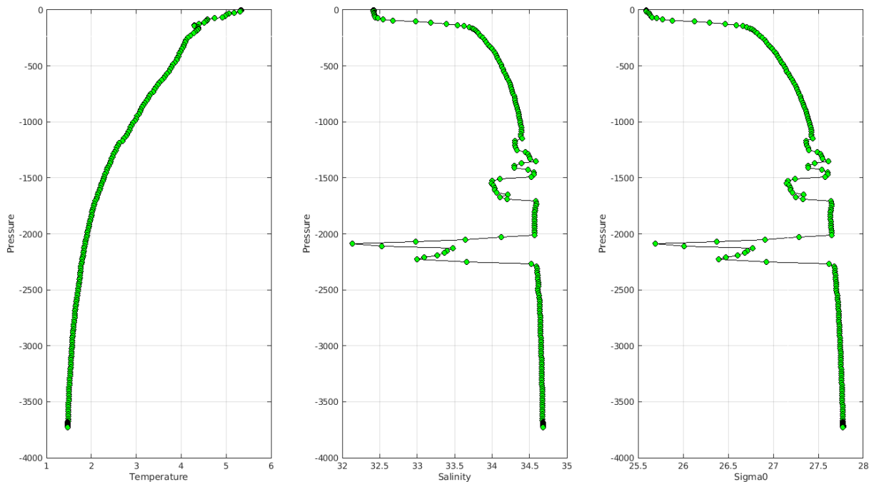
Warning MinMax Anomalies 2024 April TEMP PSAL : DAC ME- Float 4902636 - 27
