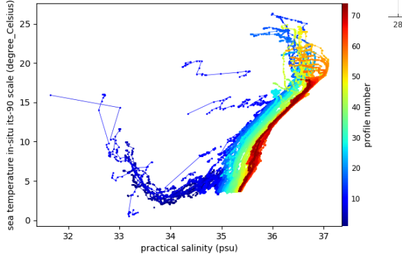
Argo float 4902595 between 19/04/2022 and 05/05/2024
