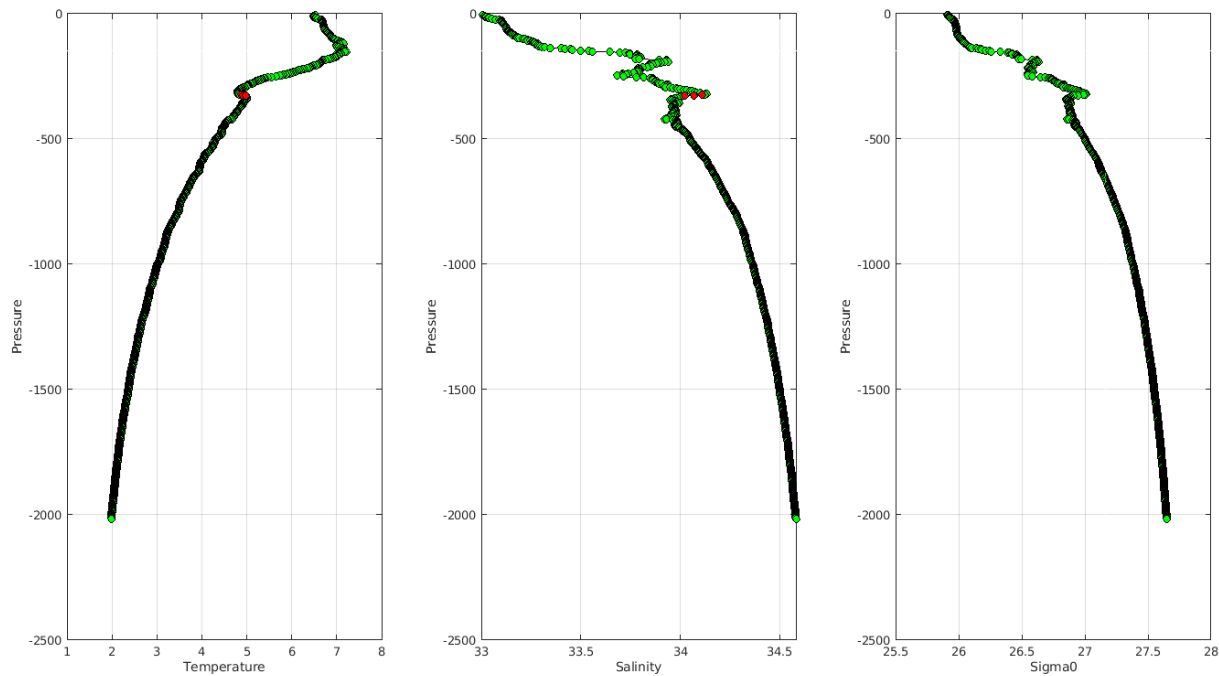
Warning MinMax Anomalies 2024 April TEMP PSAL : DAC JA- Float 4902991 - 100
