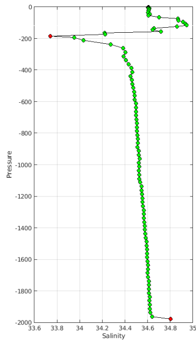
Warning MinMax Anomalies 2024 April TEMP PSAL : DAC HZ- Float 2902803 - 169
