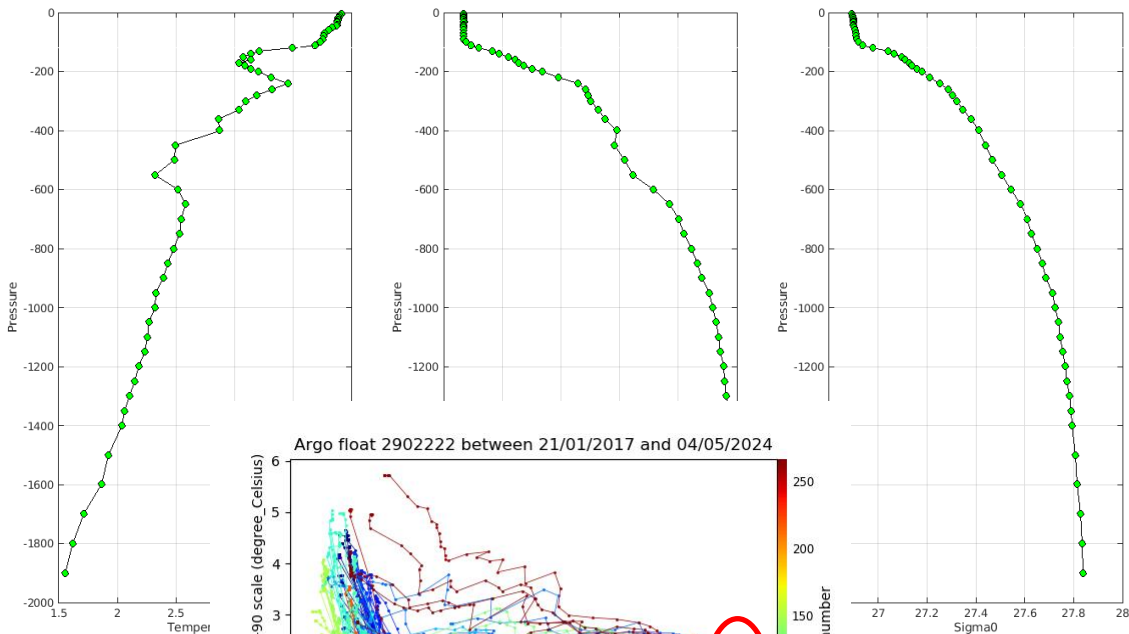
Warning MinMax Anomalies 2024 April TEMP PSAL : DAC IN- Float 2902222 - 266
