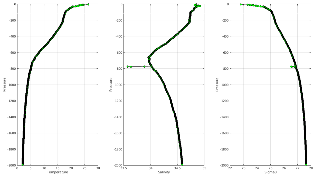
Warning MinMax Anomalies 2024 April TEMP PSAL : DAC JA- Float 2903656 - 5
