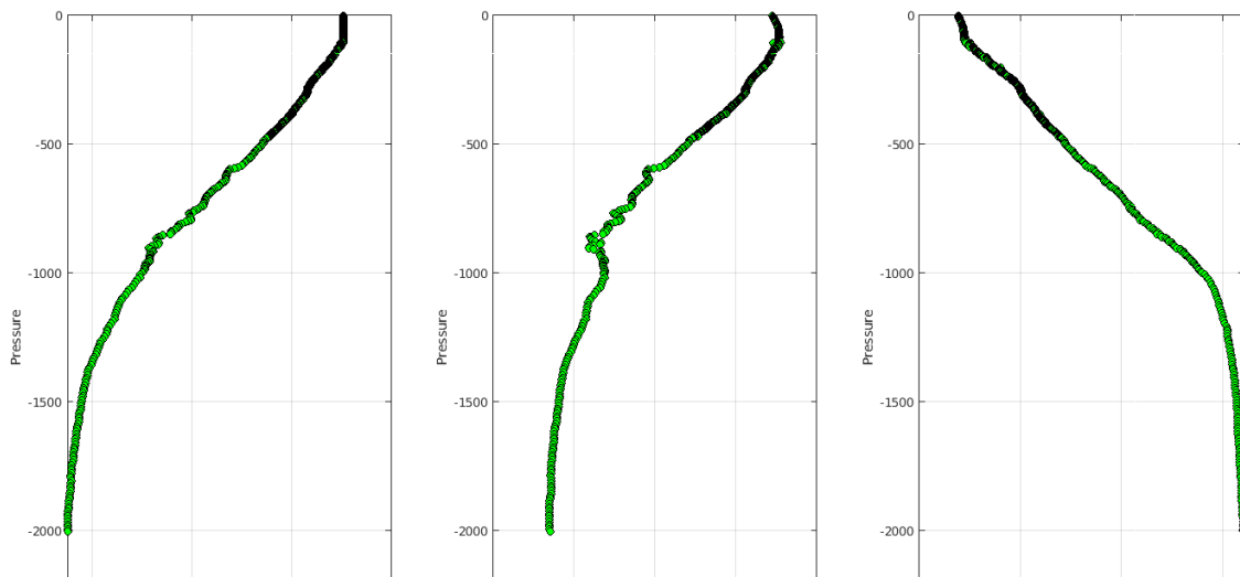
Argo float 4902595 between 19/04/2022 and 05/05/2024
