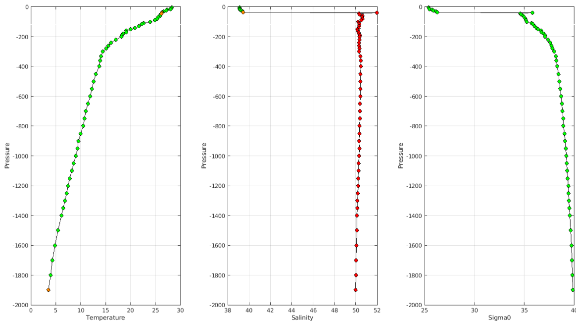
Warning MinMax Anomalies 2024 April TEMP PSAL : DAC IN- Float 2902201 - 296
