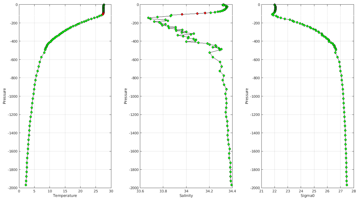
Warning MinMax Anomalies 2024 April TEMP PSAL : DAC KO- Float 3902470 - 53
