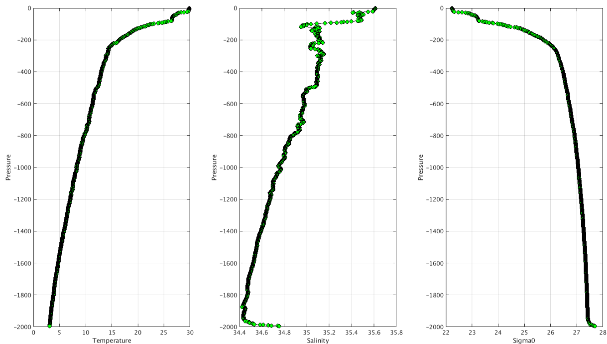
Warning MinMax Anomalies 2025 February TEMP PSAL : DAC IN- Float 2902175 - 292
