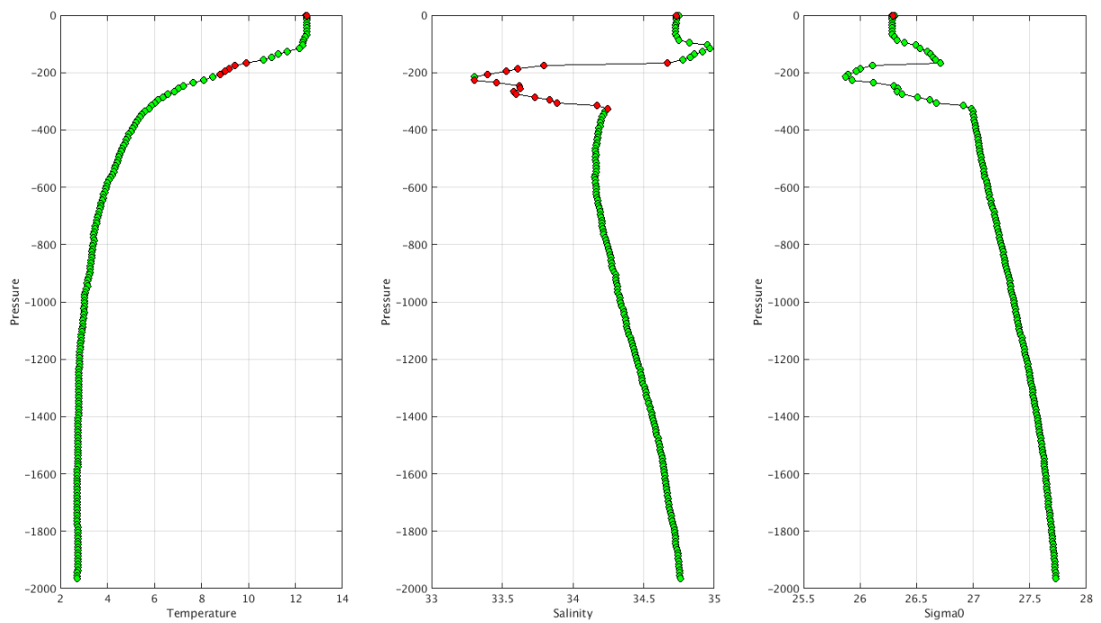
Warning MinMax Anomalies 2025 February TEMP PSAL : DAC HZ- Float 2902835 - 55
