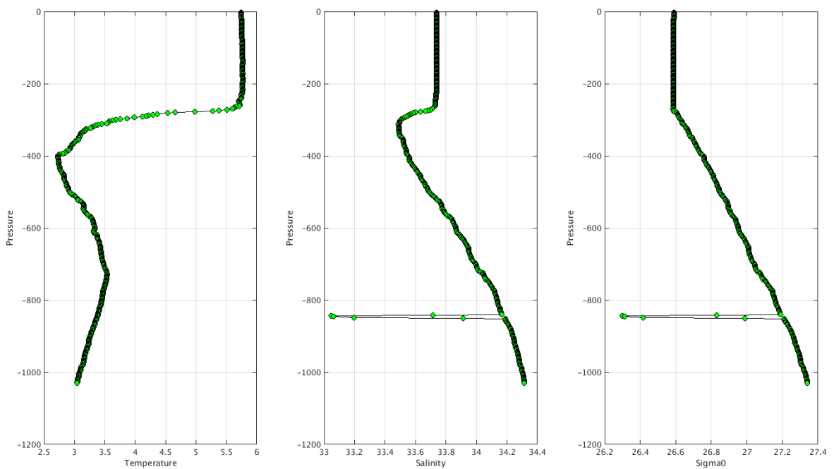
Warning MinMax Anomalies 2025 February TEMP PSAL : DAC JA- Float 2903171 - 16
