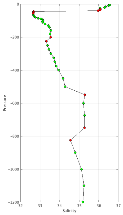
Warning MinMax Anomalies 2025 February TEMP PSAL : DAC AO- Float 2901431 - 141
