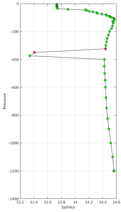
Warning MinMax Anomalies 2025 February TEMP PSAL : DAC AO- Float 2901135 - 11
