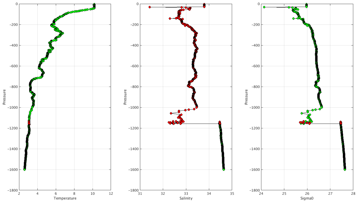
Warning MinMax Anomalies 2025 February TEMP PSAL : DAC CS- Float 1901139 - 155
