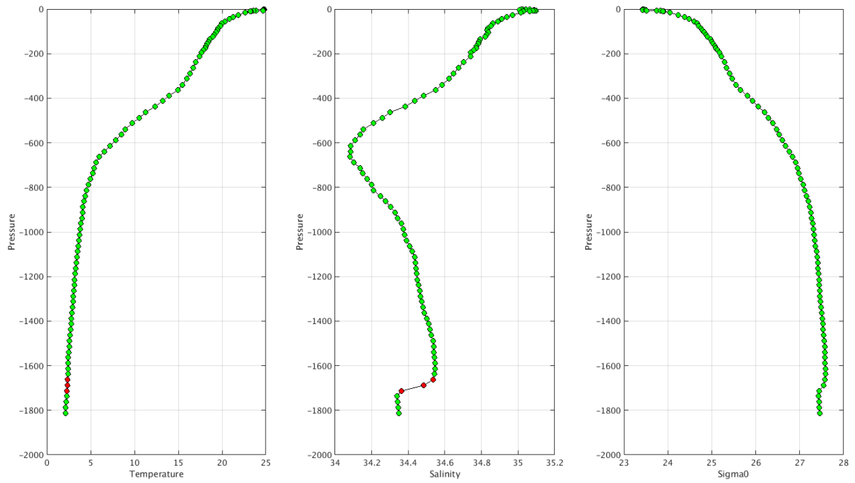
Warning MinMax Anomalies 2025 February TEMP PSAL : DAC HZ- Float 2901551 - 230
