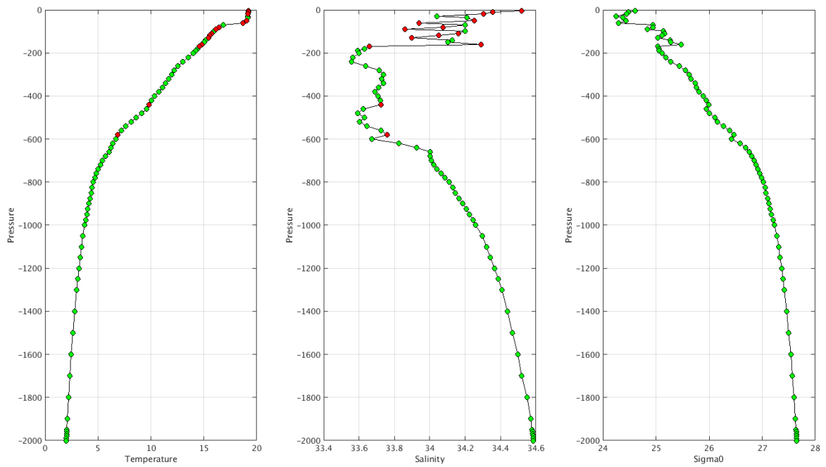
Warning MinMax Anomalies 2025 February TEMP PSAL : DAC JA- Float 2902514 - 257
