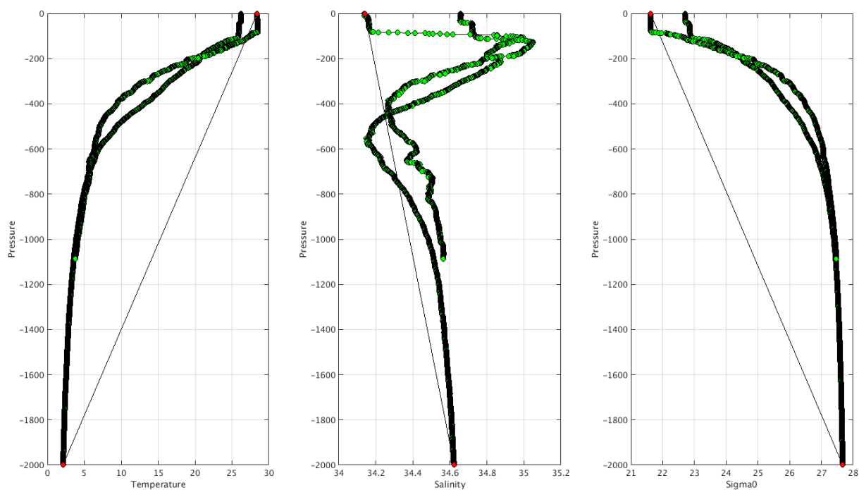
Warning MinMax Anomalies 2025 February TEMP PSAL : DAC KO- Float 4903824 - 15
