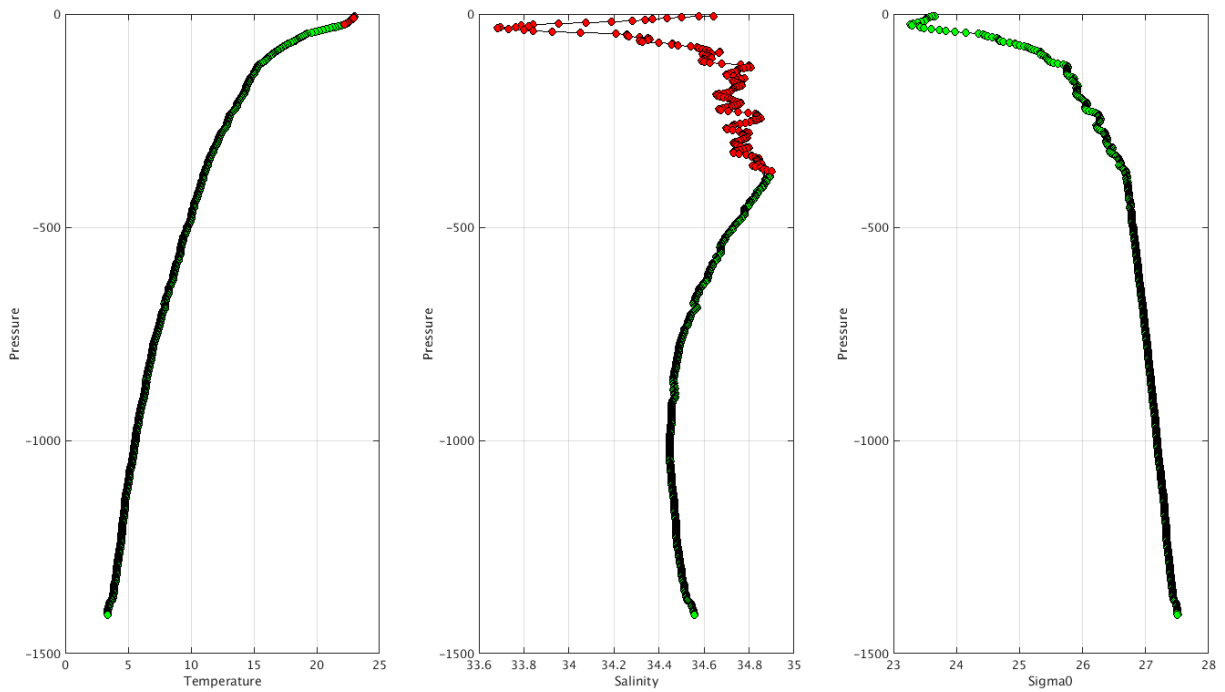
Warning MinMax Anomalies 2025 February TEMP PSAL : DAC CS- Float 5905507 - 106
