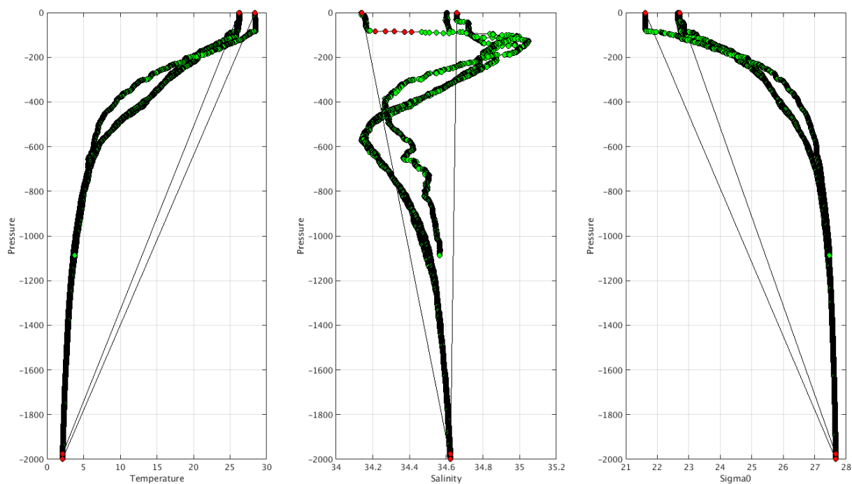
Warning MinMax Anomalies 2025 February TEMP PSAL : DAC KO- Float 2903935 - 17
